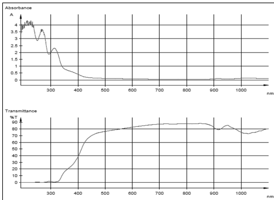
Fig 4: UV-Visible Spectra of tris(2-((E)-1-hydrazonoethyl)-4,5-dimethylphenoxy)iron
