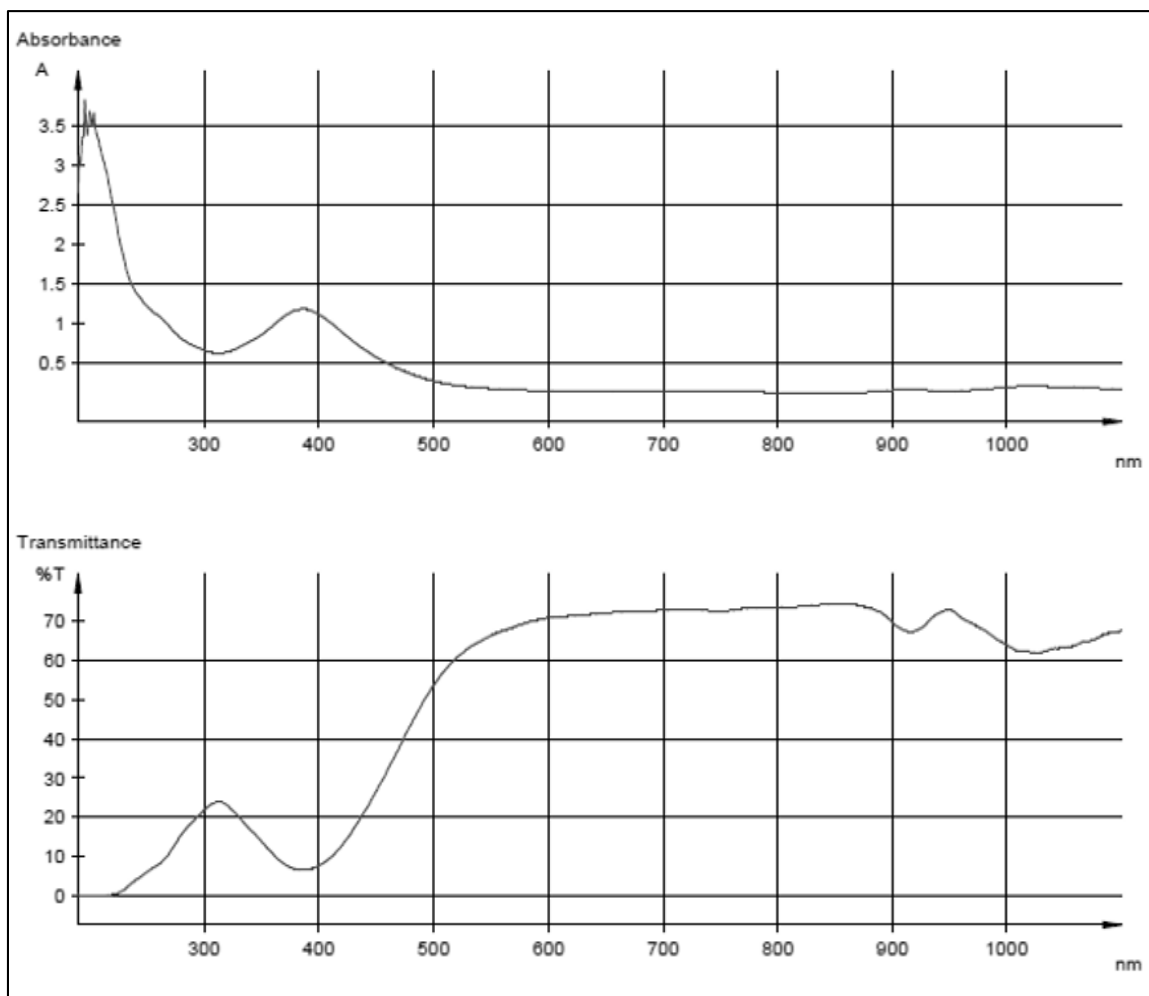
Fig 6: UV-Visible Spectra of tris(2-((E)-1-(2-(2,4-dinitrophenyl)hydrazono)ethyl)-4,5-dimethylphenoxy)iron
