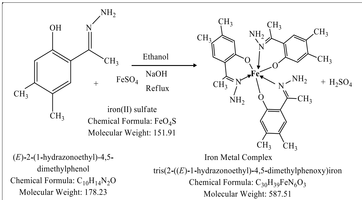
Scheme 1: Reaction scheme preparation of tris (2-(( E )-1-hydrazonoethyl)-4,5-dimethyl phenoxy)iron.
