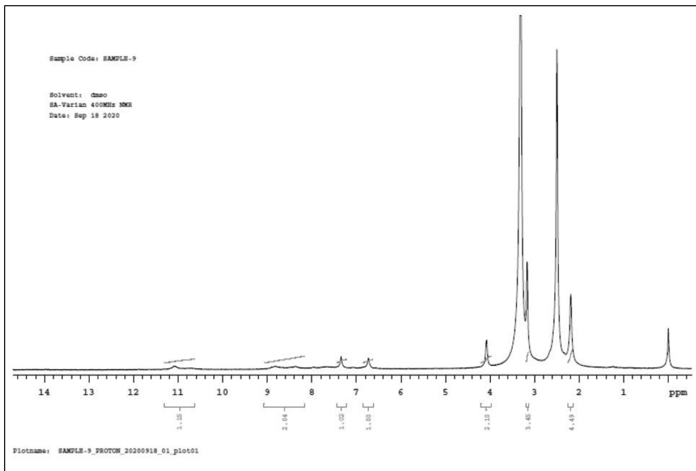
Fig 9: ^1\text{H} NMR of tris (2-((E)-1-(2-(2,4-dinitrophenyl)hydrazono)ethyl)-4,5-dimethyl phenoxy) iron
