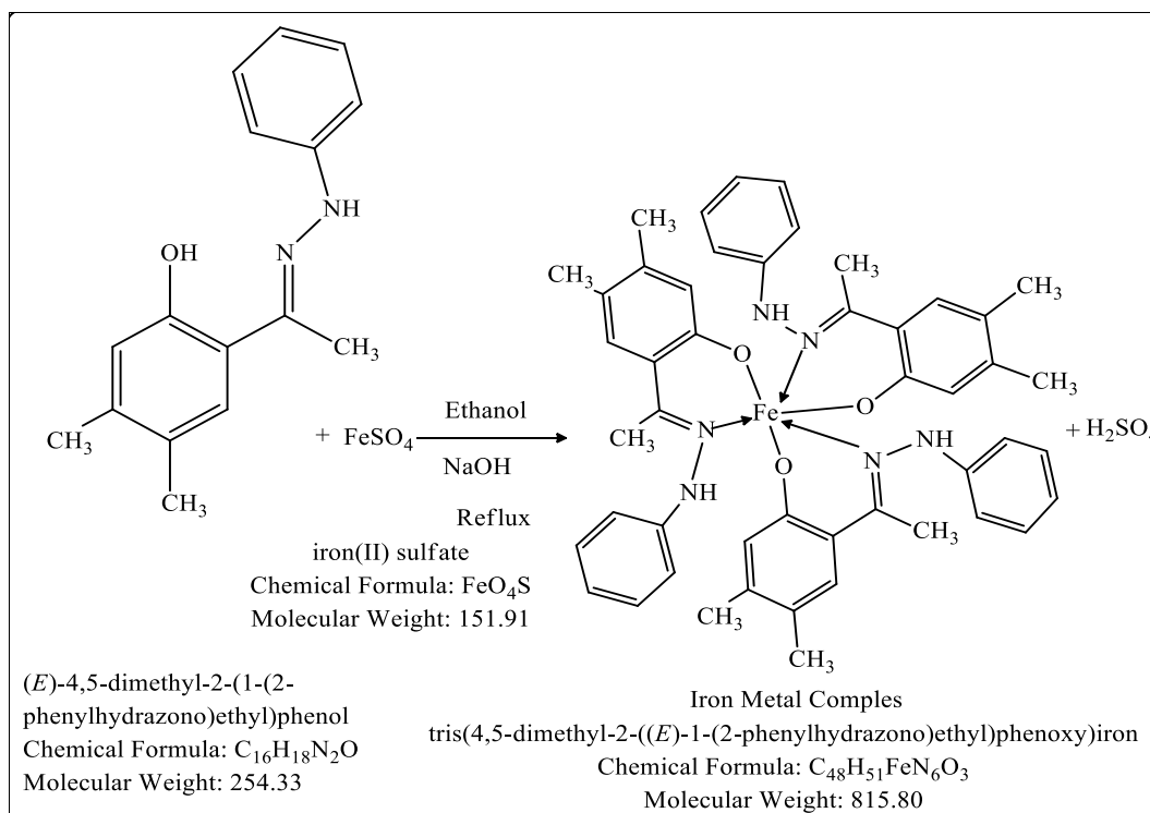
Scheme 2: Reaction scheme preparation of tris(4,5-dimethyl-2-(( E )-1-(2-phenyl hydrazono)ethyl)phenoxy)iron
