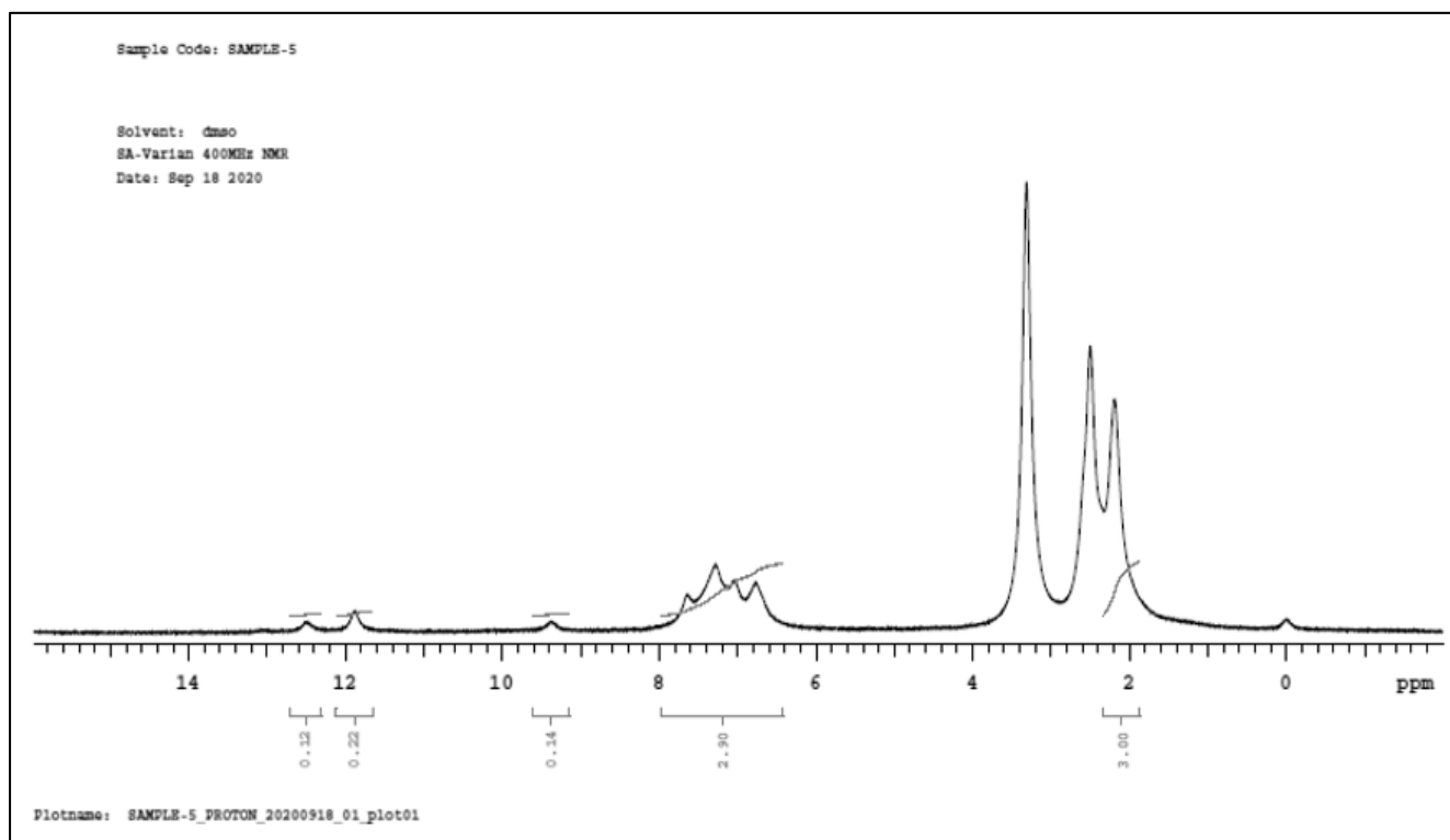
Fig 8: ^1\text{H} NMR of tris(4,5-dimethyl-2-((E)-1-(2-phenylhydrazone)ethyl) phenoxy)iron.
