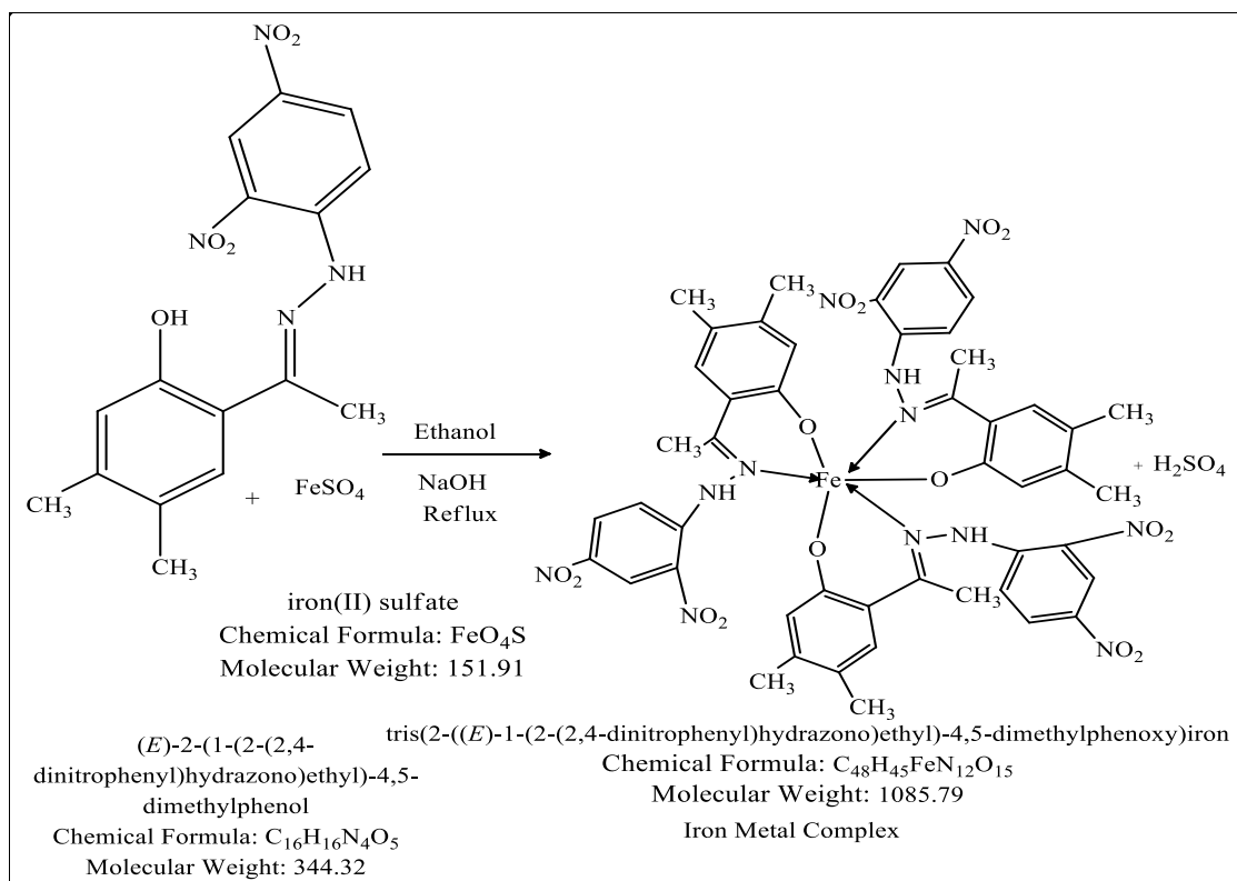
Scheme 3: Reaction scheme preparation of tris(2-((E)-1-(2-(2,4-dinitrophenyl) hydrazono)ethyl)-4,5-dimethylphenoxy)iron.
